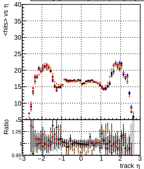
DQM_testMkFitFit_initialStepReso DQM_testMkFitFit_initialStepReso DQM_testMkFitFit_initialStepReso_wRejection5 mean hits
