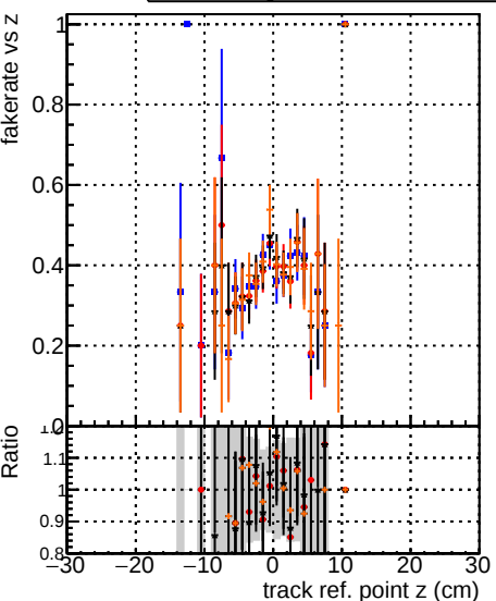
Fake rate vs v DOM original4 DOM testIMKFit_initialStepReso DOM testIMKFit_initialStepReso wRejection5 DOM testIMKFit_initialStepReso
