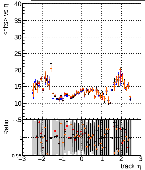
mean hit DQM_original4 DQM_testMkFit_initialStepReso DQM_testMkFitFit_initialStepReso DQM_testMkFitFit_initialStepReso_wRejection5
