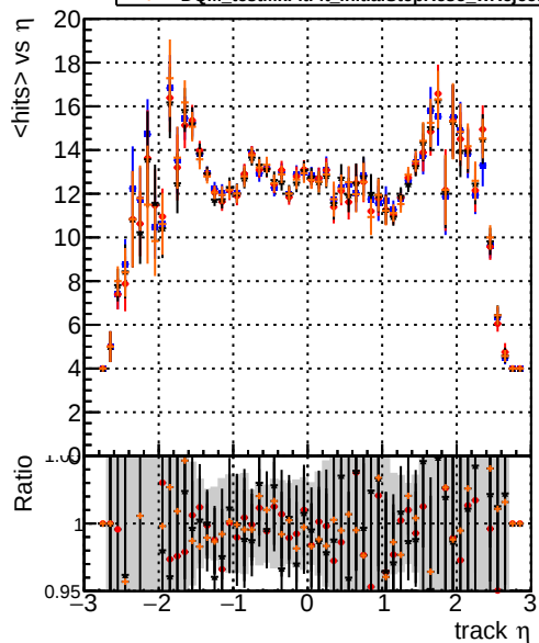
mean hit Legend: DQM_original4 (blue line) DQM_testMkFit_initialStepReso (red line with error bars) DQM_testMkFitFit_initialStepReso (black line with error bars) DQM_testMkFitFit_initialStepReso_wRejection5 (orange line with error bars)
