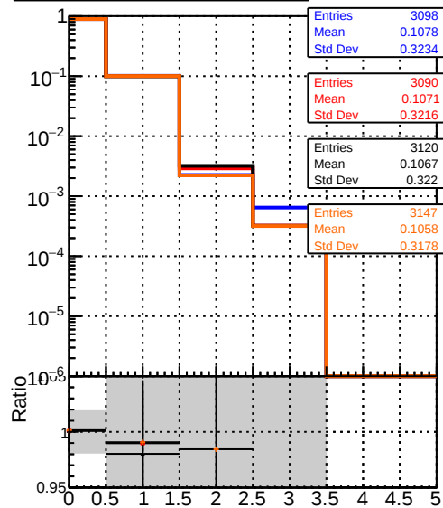
mean hit Legend: DQM_original4 (blue line) DQM_testMkFit_initialStepReso (red line with error bars) DQM_testMkFitFit_initialStepReso (black line with error bars) DQM_testMkFitFit_initialStepReso_wRejection5 (orange line with error bars)
