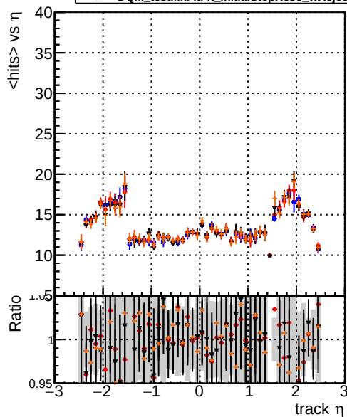
mean hit DQM_original4 DQM_testMkFitFit_initialStepReso DQM_testMkFitFit_initialStepReso_wRejection5
