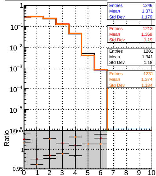
mean hit DQM_original4 DQM_testMkFitFit_initialStepReso DQM_testMkFitFit_initialStepReso_wRejection5
