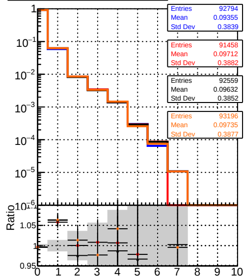
mean hit DQM_testMkFit_initialStepReso DQM_testMkFitFit_initialStepReso DQM_testMkFitFit_initialStepReso_wRejection5
