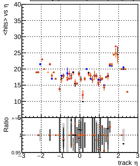
mean hit DQM_original4 DQM_testMkFit_initialStepReso DQM_testMkFitFit_initialStepReso DQM_testMkFitFit_initialStepReso_wRejection5
