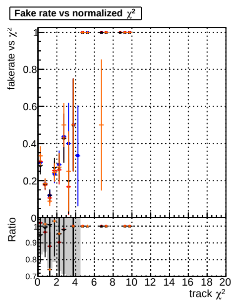
Fake rate vs. Legend: DOM original4 DOM testMKFit_InitialStepReso DOM testMKFit_InitialStepReso wRejection5 DOM testMKFit_InitialStepReso
