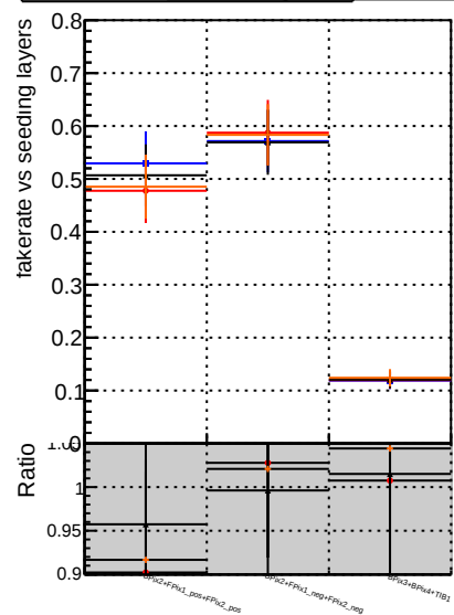
Fake rate vs. Legend: DOM original4 DOM testMKFit_InitialStepReso DOM testMKFit_InitialStepReso wRejection5 DOM testMKFit_InitialStepReso
