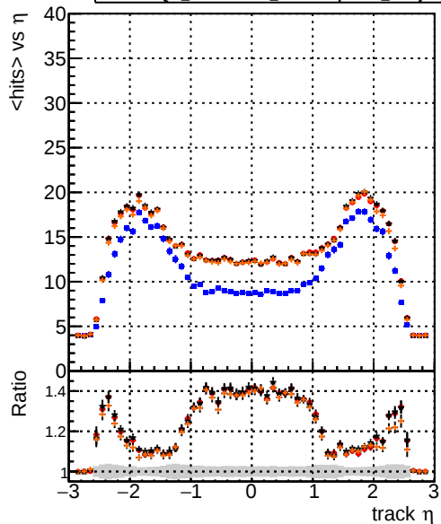
mean hits vs \eta Legend: DQM_original4 (blue line), DQM_testMkFit_initialStepReso (red line with dots), DQM_testMkFitFit_initialStepReso (black line with dots), DQM_testMkFitFit_initialStepReso_wRejection5 (orange line with dots)
