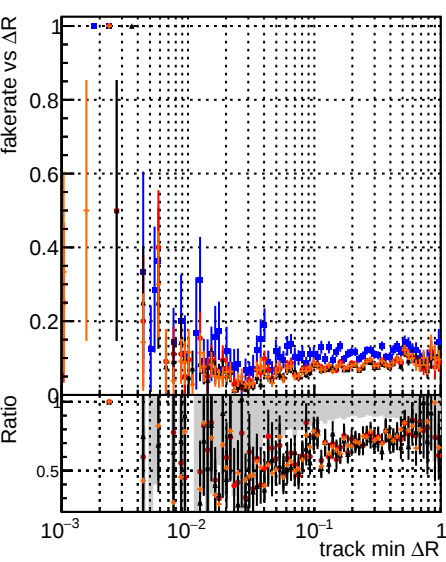
Fake rate vs \Delta R(\text{track, jet}) DOM original DOM test DOM fit initialStepReso DOM fit initialStepReso wRejection5
