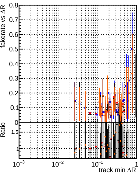
Fake rate vs ΔR(track, jet) Legend: DOM original (blue) DOM test (red) DOM MC Fit initialStepReso (black) DOM MC Fit initialStepReso wRejection5 (orange)
