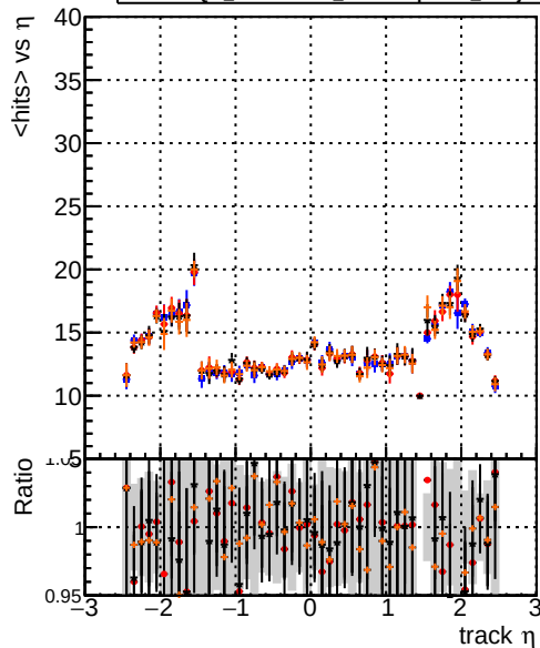
mean hit — DQM_original4 — DQM_testMkFit_fit_initialStepReso — DQM_testMkFitFit_initialStepReso — DQM_testMkFitFit_initialStepReso_wRejection5
