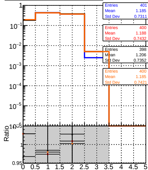
mean hit DQM_original4 DQM_testMkFit_fit_initialStepReso DQM_testMkFitFit_initialStepReso DQM_testMkFitFit_initialStepReso_wRejection5
