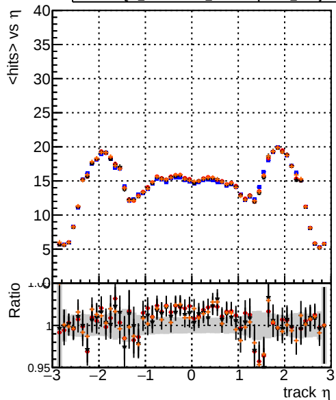
mean hit DQM_origina14 DQM_testMkFit_initialStepReso DQM_testMkFitFit_initialStepReso DQM_testMkFitFit_initialStepReso_wRejection5
