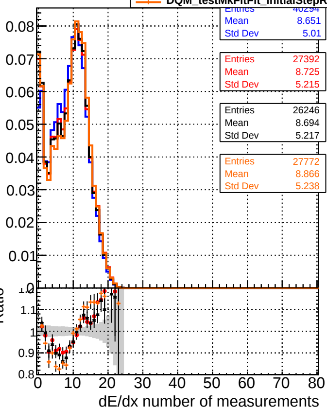
— DQM_original4 — DQM_testMkFit_initialStepReso — DQM_testMkFitFit_initialStepReso — DQM_testMkFitFit_initialStepReso_wRejection5
