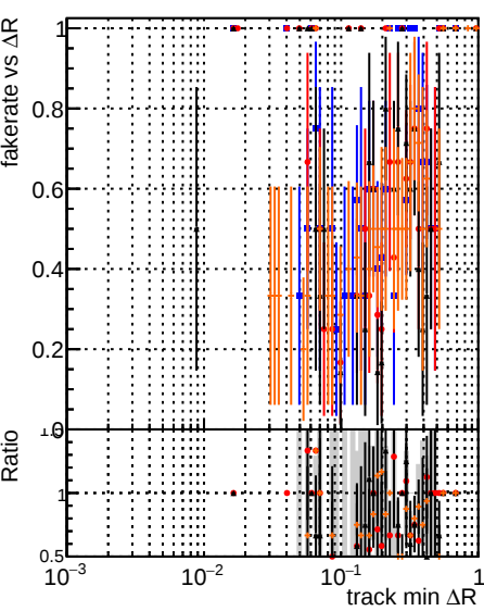
Fake rate vs \Delta R(\text{track, jet}) DQM original4 DQM Fit initialStepReso DQM Fit initialStepReso DQM Fit initialStepReso wRejection5
