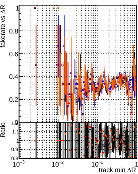
Fake rate vs \Delta R(\text{track, jet}) DOM original4 DOM test4 DOM test4 wRejection5 DOM test4 initialStepReso DOM test4 MKFit initialStepReso DOM test4 MKFit initialStepReso DOM test4 MKFit initialStepReso
