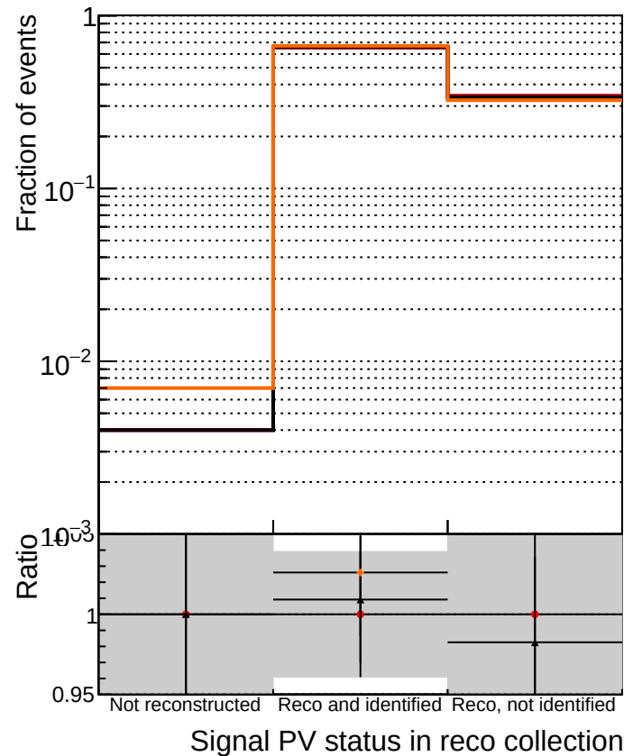
DQM_original4 DQM_testMkFitFit_initialStepReso DQM_testMkFitFit_initialStepReso DQM_testMkFitFit_initialStepReso_wRejection5
