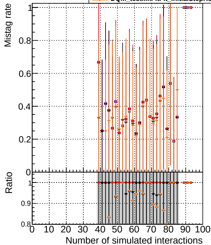
DQM_original4 DQM_testMkFitFit_initialStepReso DQM_testMkFitFit_initialStepReso DQM_testMkFitFit_initialStepReso_wRejection5
