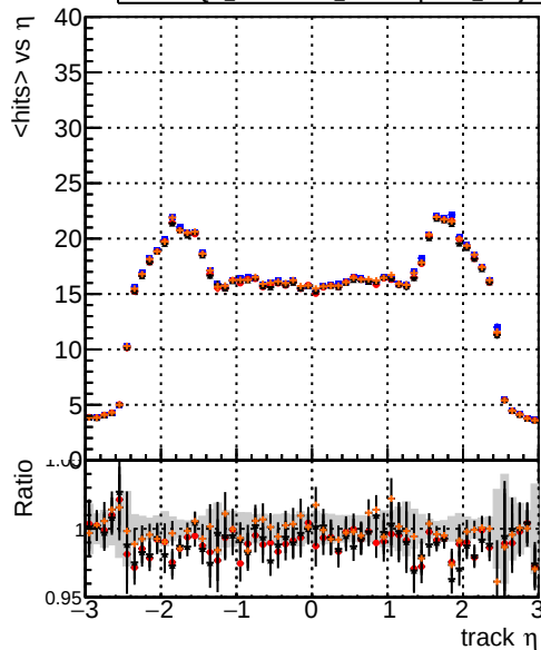
mean hit DQM_original4 DQM_testMkFit_initialStepReso DQM_testMkFitFit_initialStepReso DQM_testMkFitFit_initialStepReso_wRejection5
