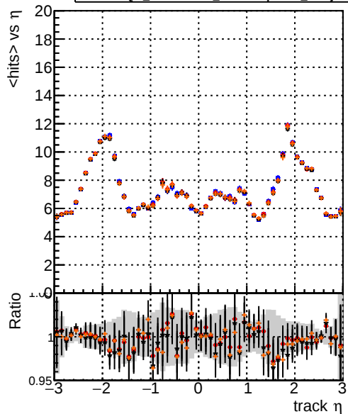
mean hits — DQM_original4 — DQM_testMkFit_fit_initialStepReso — DQM_testMkFitFit_initialStepReso — DQM_testMkFitFit_initialStepReso_wRejection5
