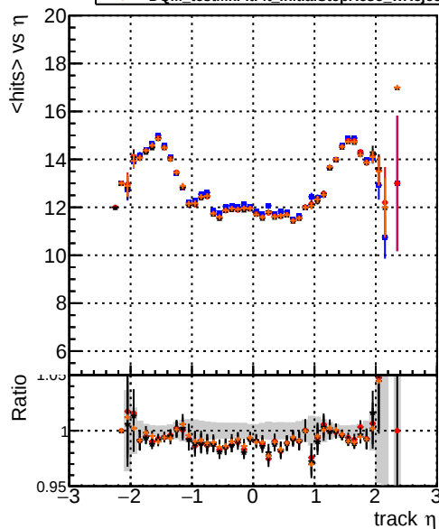
mean hits vs \eta Legend: Blue line: DQM_original4 Red line: DQM_testMkFit_initialStepReso Black line: DQM_testMkFitFit_initialStepReso Orange line: DQM_testMkFitFit_initialStepReso_wRejection5
