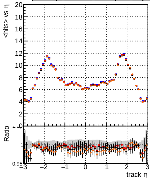
mean hit DQM_original DQM_testMkFit_initialStepReso DQM_testMkFitFit_initialStepReso DQM_testMkFitFit_initialStepReso_wRejection5
