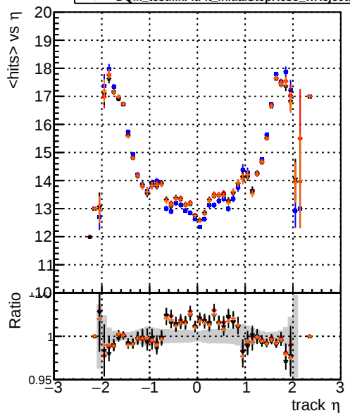
mean hits vs \eta Legend: DQM_testMkFit_initialStepReso (blue line), DQM_testMkFitFit_initialStepReso (red line), DQM_testMkFitFit_initialStepReso_wRejection5 (black line)
