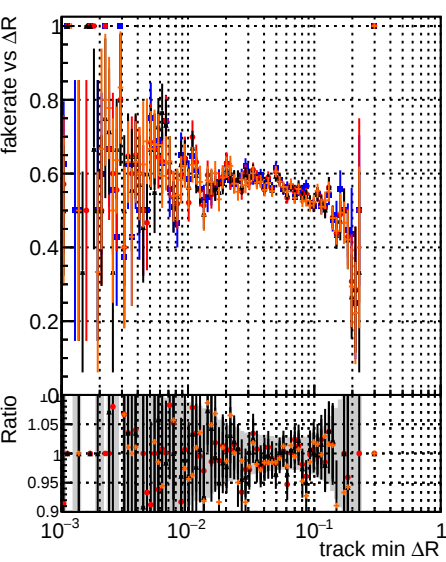
Fake rate vs \Delta R(\text{track, jet}) DOM original4 DOM testIMKFit_initialStepReso DOM testIMKFit_initialStepReso_wRejection5
