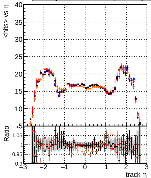
— DQM_testMkFitFit_initialStepReso — DQM_testMkFitFit_initialStepReso — DQM_testMkFitFit_initialStepReso — DQM_testMkFitFit_initialStepReso_wRejection5 mean hits
