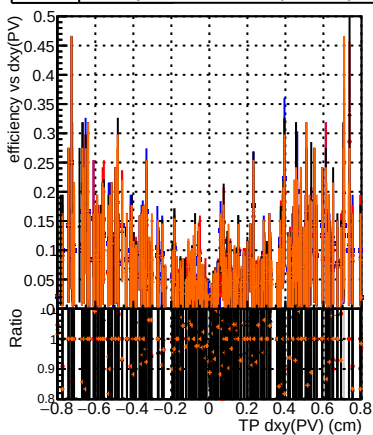
Efficiency —●— DQM_testMkFitIt-It_initialStepReso —●— DQM_testMkFitFit_initialStepReso_wRejection10
