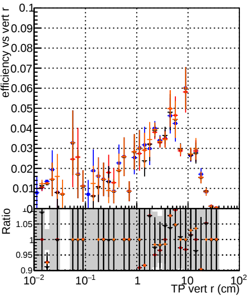
Efficiency vs TP vert r (cm) DQM_original4 DQM_testMkFit_initialStepReso DQM_testMkFitFit_initialStepReso DQM_testMkFitFit_initialStepReso_wRejection10
