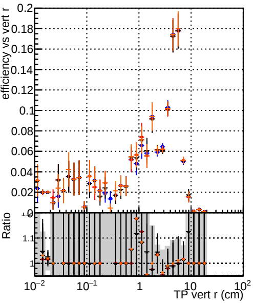
Efficiency vs vertpos Legend: DQM_original4 DQM_testMkFit_initialStepReso DQM_testMkFitFit_initialStepReso DQM_testMkFitFit_initialStepReso_wRejection10
