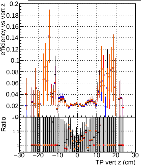
Efficiency vs vertpos Legend: DQM_original4 DQM_testMkFit_initialStepReso DQM_testMkFitFit_initialStepReso DQM_testMkFitFit_initialStepReso_wRejection10
