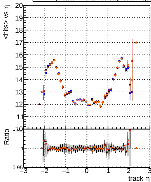
DQM_testMkFit_initialStepReso DQM_testMkFitFit_initialStepReso DQM_testMkFitFit_initialStepReso_wRejection10 mean hits
