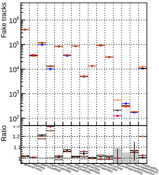
Number — DQM original — DQM testMkFit_initialStepReso — DQM testMkFitFit_initialStepReso — DQM testMkFitFit_initialStepReso wRejection10
