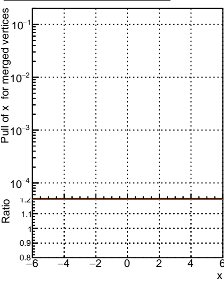
RecoAllAssoc2GenMatchedMerged_PullX
