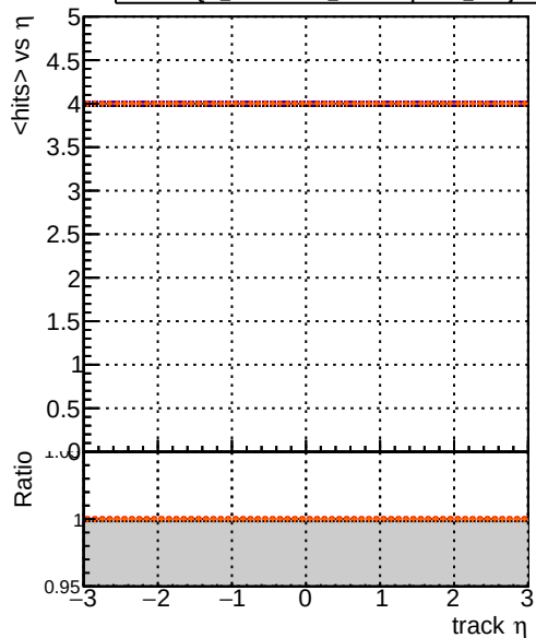
DQM_original14 DQM_testMkFit_initialStepReso DQM_testMkFitFit_initialStepReso DQM_testMkFitFit_initialStepReso_wRejection10 mean hits
