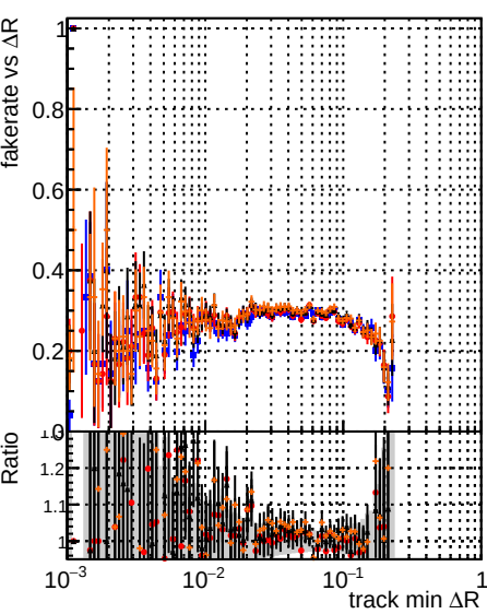
Fake rate vs \Delta R(\text{track, jet}) DQM original4 DQM techIMKFit_initialStepReso DQM techIMKFit_initialStepReso wRejection10
