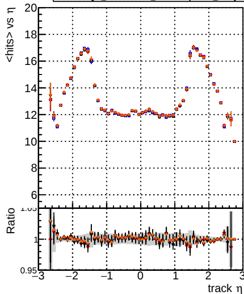
DQM_original4 DQM_testMkFit_fit_initialStepReso DQM_testMkFitFit_initialStepReso DQM_testMkFitFit_initialStepReso_wRejection10 mean hit
