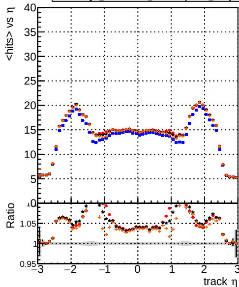
mean hits DQM_original DQM_testMkFit_initialStepReso DQM_testMkFitFit_initialStepReso DQM_testMkFitFit_initialStepReso_wRejection10
