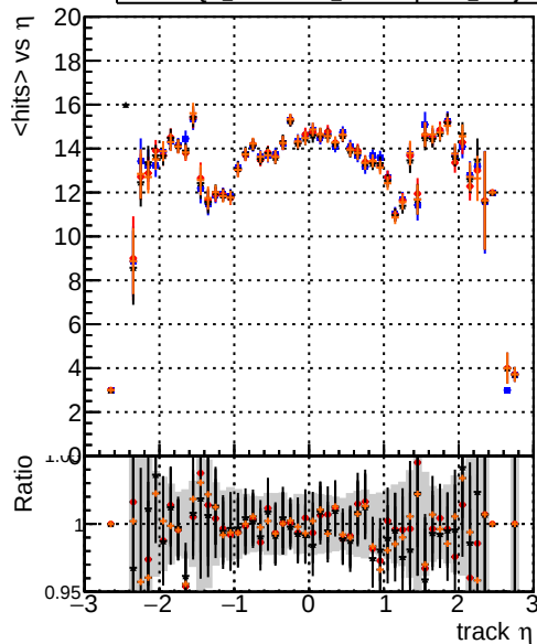
Legend: — DQM_original4 — DQM_testMkFit_initialStepReso — DQM_testMkFitFit_initialStepReso — DQM_testMkFitFit_initialStepReso_wRejection10 mean hit
