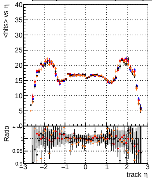
mean hit DQM_original4 DQM_testMkFit_initialStepReso DQM_testMkFitFit_initialStepReso DQM_testMkFitFit_initialStepReso_wRejection10
