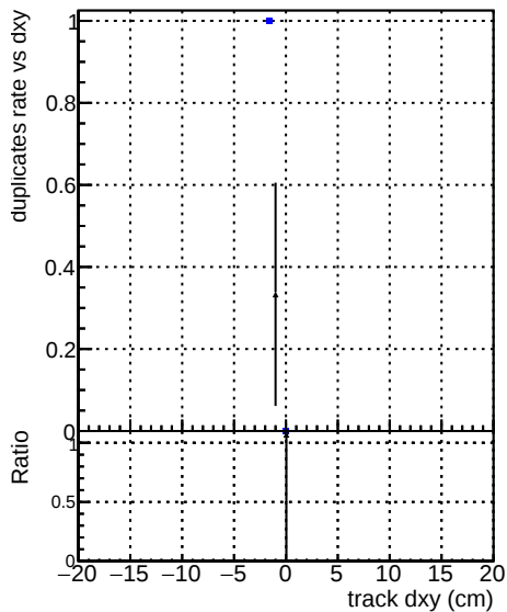
wRejection10
