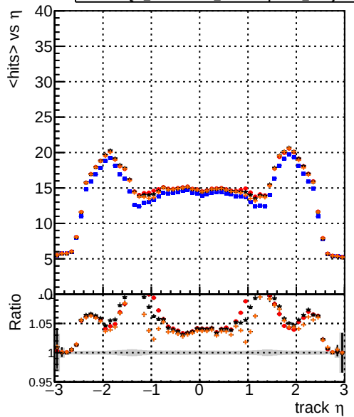
mean hit DQM_original DQM_testMkFit_initialStepReso DQM_testMkFitFit_initialStepReso DQM_testMkFitFit_initialStepReso_wRejection10
