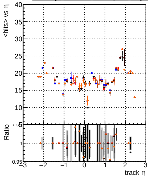
mean hit DQM_original14 DQM_testMkFit_fit_initialStepReso DQM_testMkFitFit_initialStepReso DQM_testMkFitFit_initialStepReso_wRejection10
