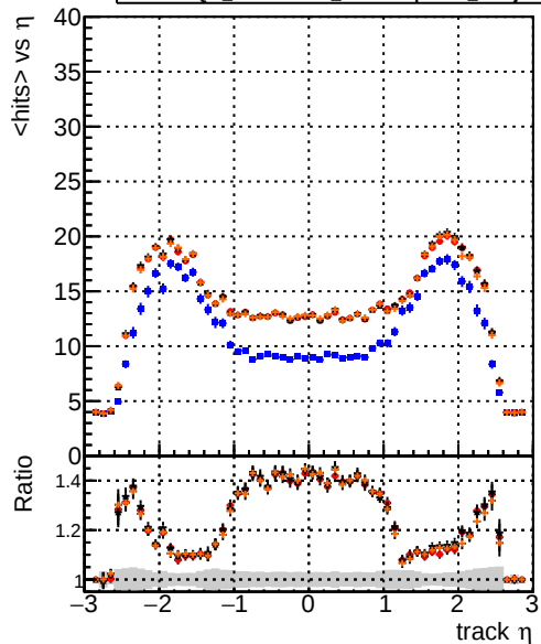
mean hit DQM_original4 DQM_testMkFit_fit_initialStepReso DQM_testMkFitFit_initialStepReso DQM_testMkFitFit_initialStepReso_wRejection10
