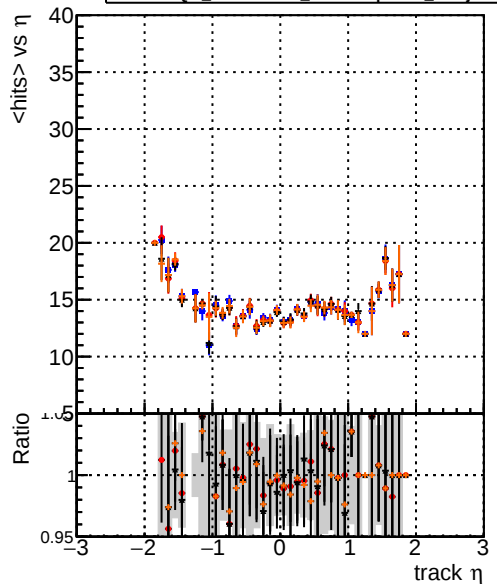
DQM_original4 DQM_testMkFit_fit_initialStepReso DQM_testMkFitFit_initialStepReso DQM_testMkFitFit_initialStepReso_wRejection10 mean hits
