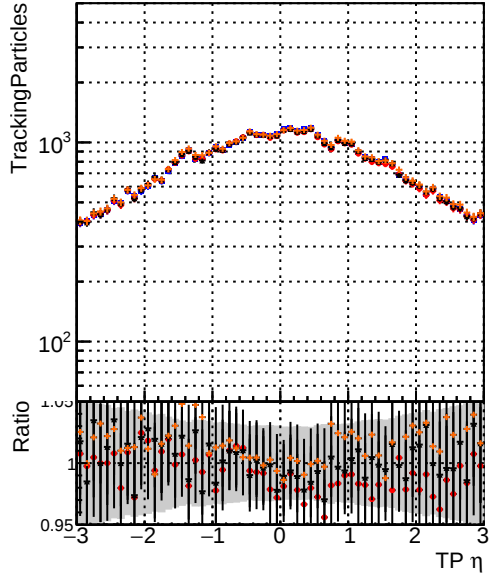
N of simulated tracks vs TP \eta Legend: DQM_original4 DQM_testMkFit_initialStepReso DQM_testMkFitFit_initialStepReso DQM_testMkFitFit_initialStepReso_wRejection10
