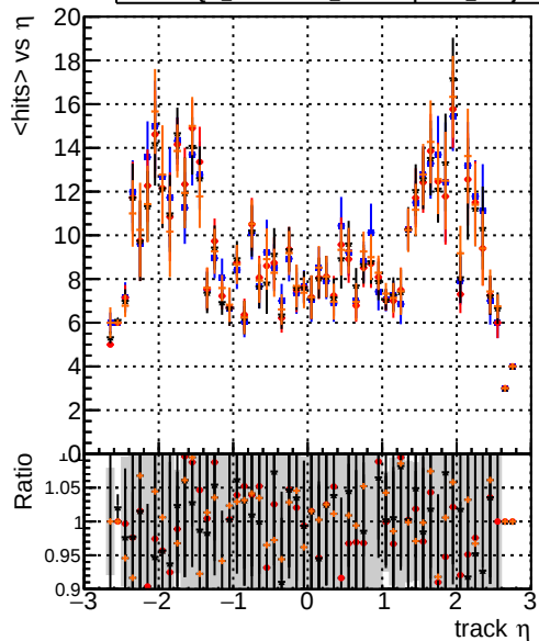
DQM_original4 DQM_testMkFit_initialStepReso DQM_testMkFitFit_initialStepReso DQM_testMkFitFit_initialStepReso_wRejection10 mean hits
