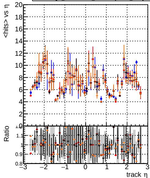
— DQM_testMkFit_initialStepReso — DQM_testMkFitFit_initialStepReso — DQM_testMkFitFit_initialStepReso_wRejection10 mean hits
