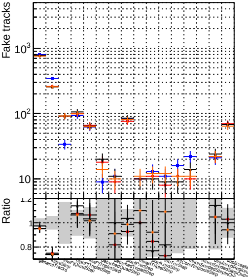
Number DQM_original4 DQM_testMkFit_initialStepReso DQM_testMkFitFit_initialStepReso DQM_testMkFitFit_initialStepReso_wRejection10
