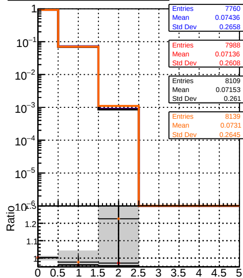
mean hit DQM_origina14 DQM_testMkFit_initialStepReso DQM_testMkFitFit_initialStepReso DQM_testMkFitFit_initialStepReso_wRejection10
