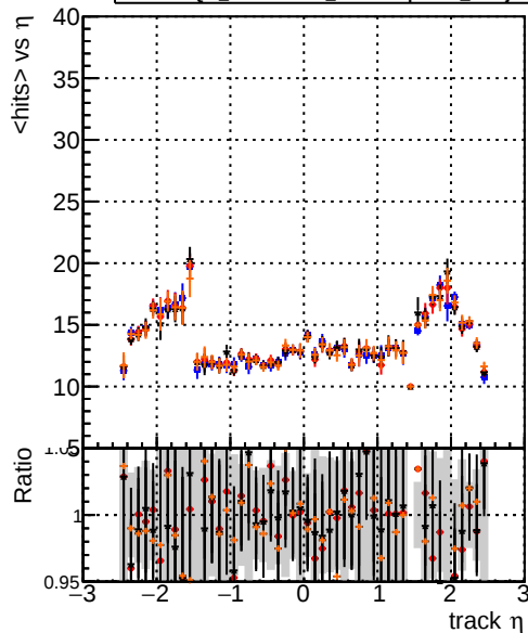
mean hit DQM_original4 DQM_testMkFit_initialStepReso DQM_testMkFitFit_initialStepReso DQM_testMkFitFit_initialStepReso_wRejection10
