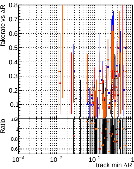
Fake rate vs ΔR(track, jet) Legend: DOM original (blue) DOM test (red) DOM fit initialStepReso (black) DOM fit initialStepReso wRejection10 (orange)
