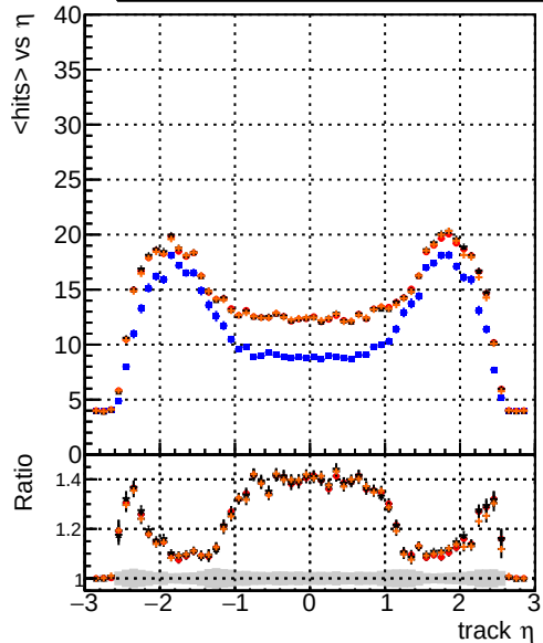
— DQM_original4 — DQM_testMkFit_initialStepReso — DQM_testMkFitFit_initialStepReso — DQM_testMkFitFit_initialStepReso_wRejection10
